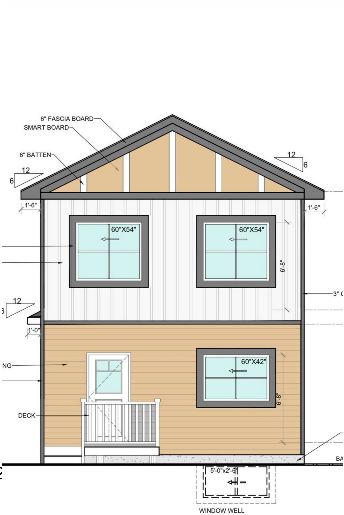
REAR ELEVATION
